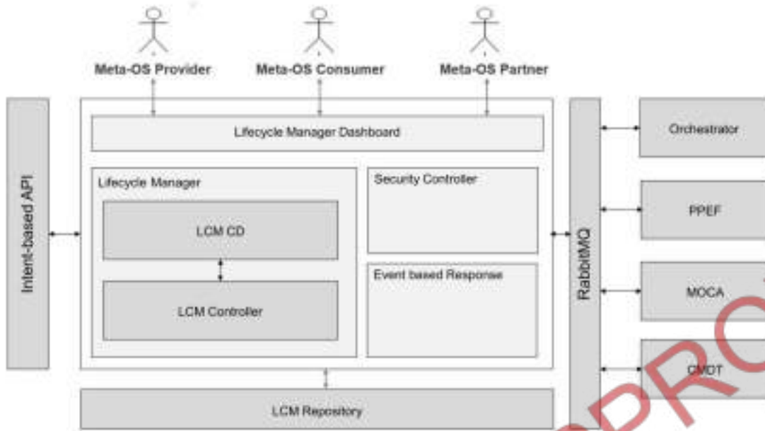
Figure 35: LCM Architecture
